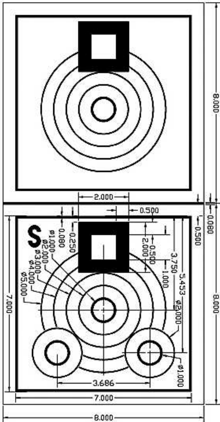
200Yd. TARGET FOR HORIZONTAL BACKERS
